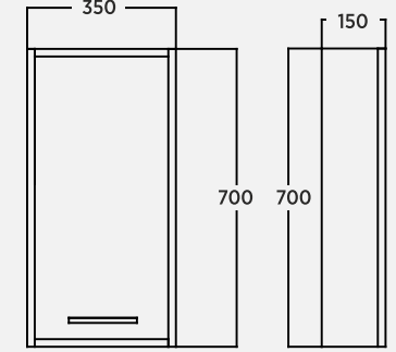
Mod 35 cm Üst Yan Dolap Upper Side Cabinet | Armadio Laterale Superior
