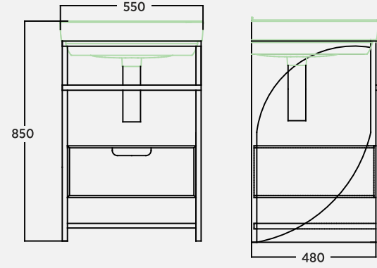
Nova 55 cm Lavabo Dolabı Washbasin Cabinet | Mobile Lavabo
